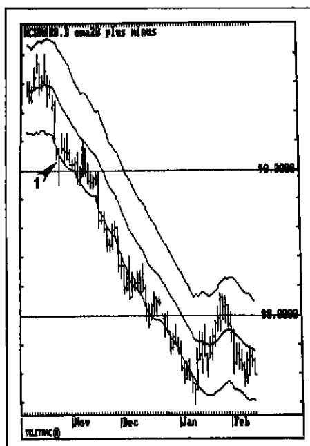
Daily copper prices with Keltner Channels
